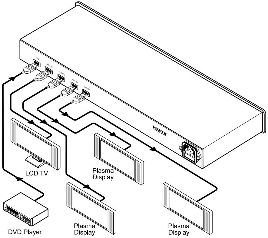
Figure 2: Connecting a VM-4HDMI 1:4 HDMI Distributor
