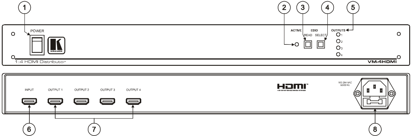
Figure 1: VM-4HDMI 1:4 HDMI Distributor
